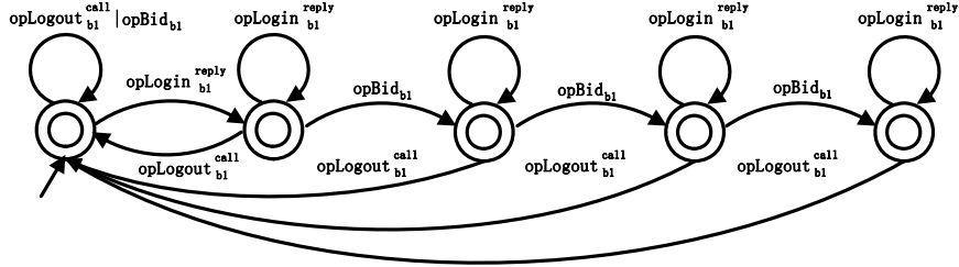
Fig. 7. FSA for the Example Interaction Constraint of Figure 5
