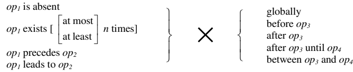
Fig. 2. Pattern and Scope Operators
