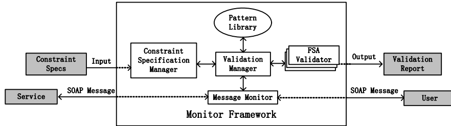
Fig. 6. Validation Framework
