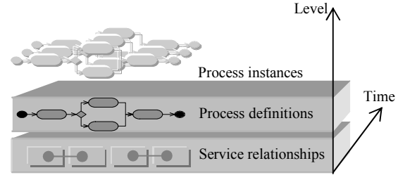
Figure 2: Levels of process flexibility
