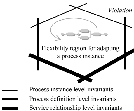
Figure 5: Boundaries of flexibility of a runtime process instance
