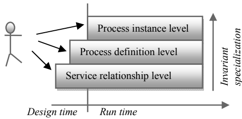
Figure 4: Invariants in all three levels of a services composition
